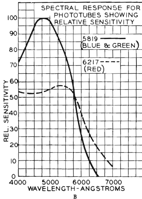
FIGS. 9A, B and C. Spectral response curves.
