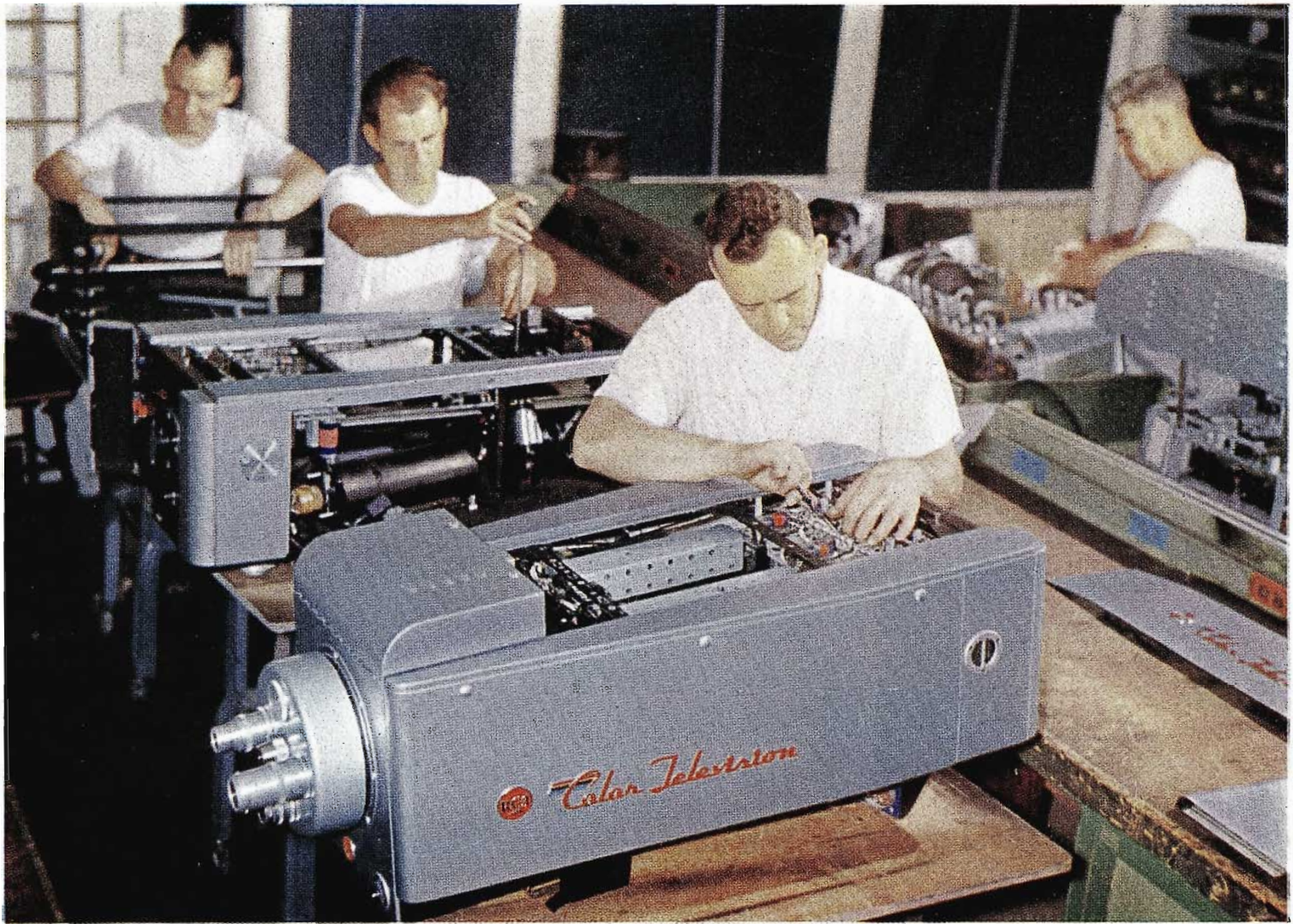
FIG. 8. Workmen assemble RCA Color Television Cameras. These cameras and other items of Color Television Broadcast Equipment have been made available to Broadcasters everywhere.
