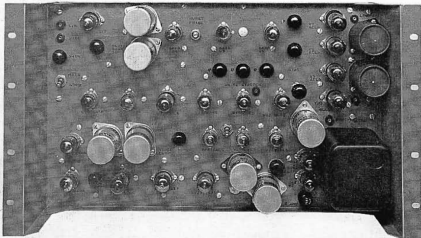
FIG. 3. RCA TA-7A Stabilizing Amplifier designed especially for color signal service.
