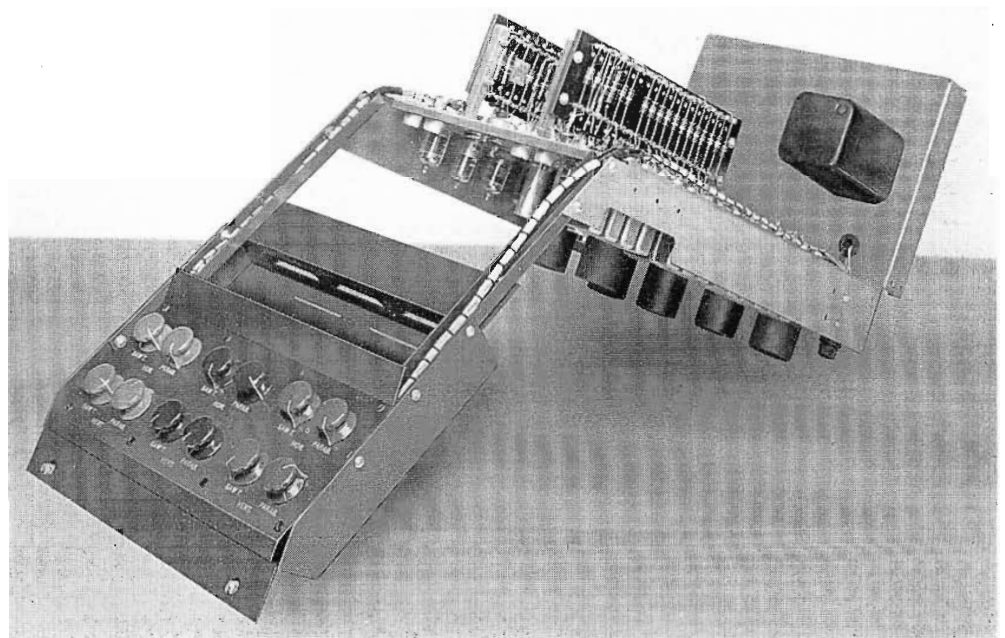
FIG. 15. Shading generator assembly with control panel.
