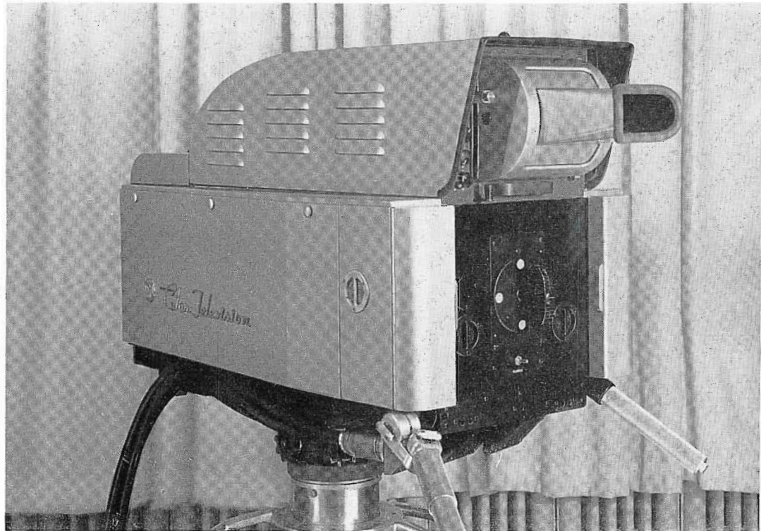
FIG. 6. Rear view of RCA Color Camera with viewing hood in place.
