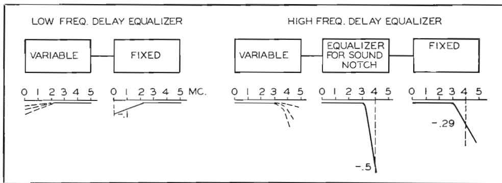
FIG. 13. Functional division of phase equalizers.
