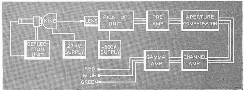
FIG. 2. Color Slide Camera unit diagram.
