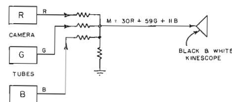
FIG. 5. Block diagram showing how a color camera may be connected to a black and white kinescope.
