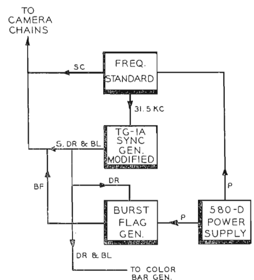
FIG. 6. Functional arrangement of equipment units for producing color sync signals locally (Equipment Group C).
