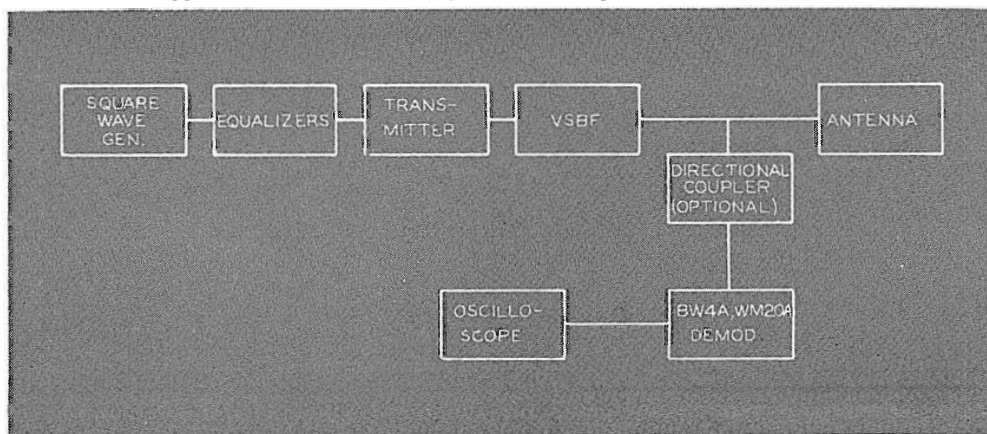
FIG. 21. Apparatus arrangement for square wave response measurement of transmitter.
