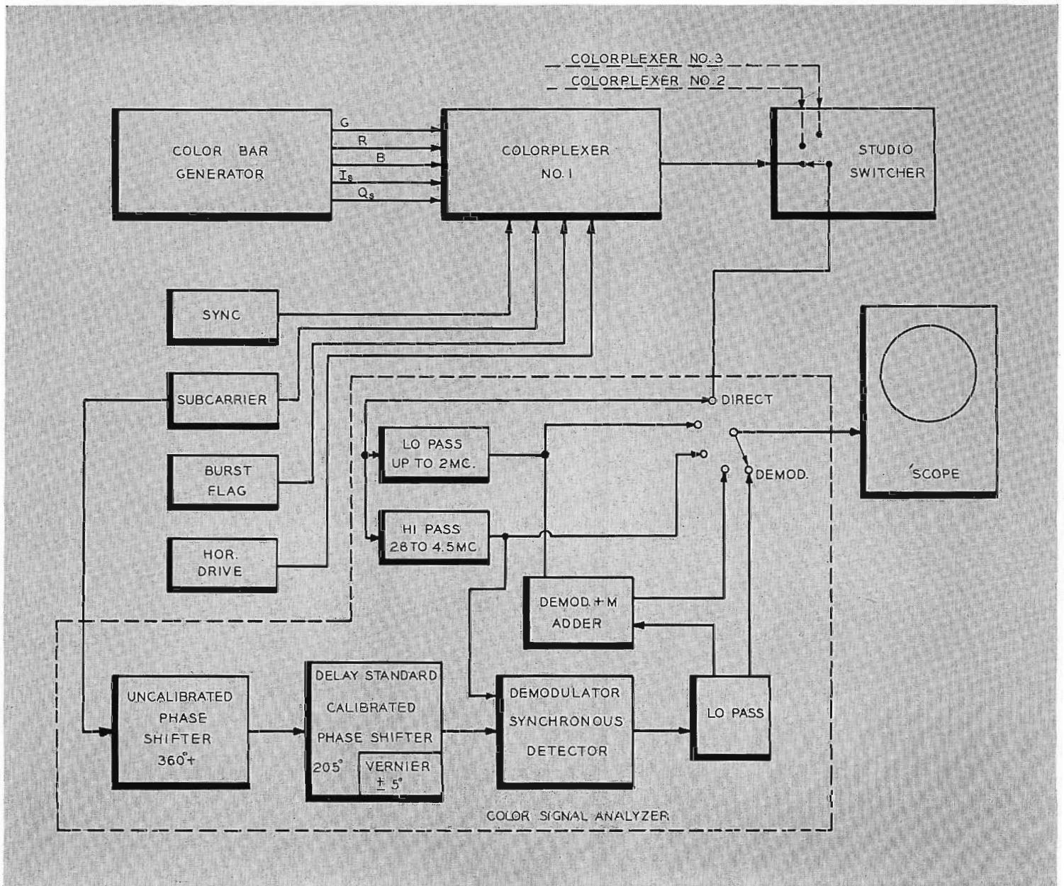
FIG. 6. Test Equipment arranged for Colorplexer alignment in order to produce a composite color television signal.
