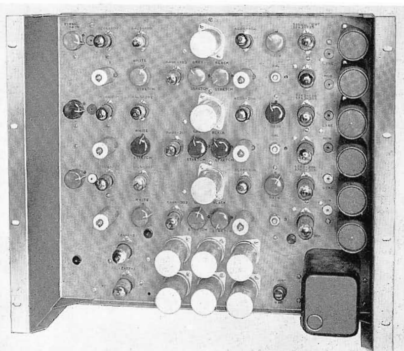
FIG. 14. Gamma Amplifier. A non-linear amplifier used to correct the video signals for the non-linear characteristics of the receiver kinescope.
