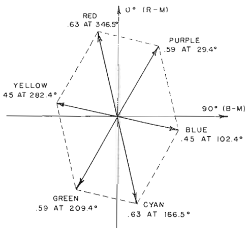
FIG. 23. Vector diagram showing the sub-carrier amplitudes and phases corresponding to six major colors.
