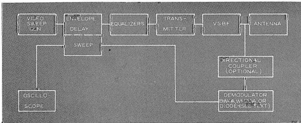
FIG. 23. Apparatus arrangement employing an envelope delay sweep for phase equalizer adjustment and measurement of transmitter envelope delay.
