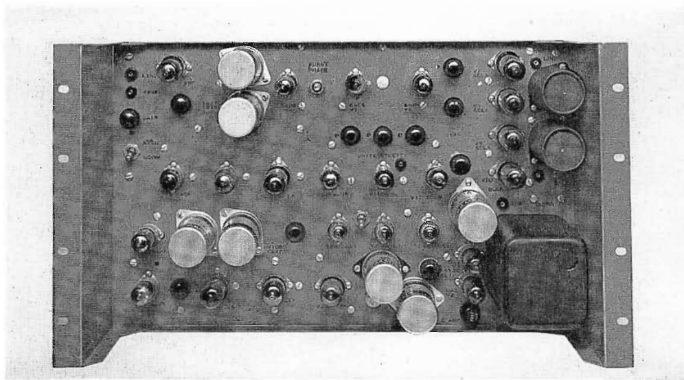
FIG. 16. Color stabilizing amplifier with built-in linearity corrector.
