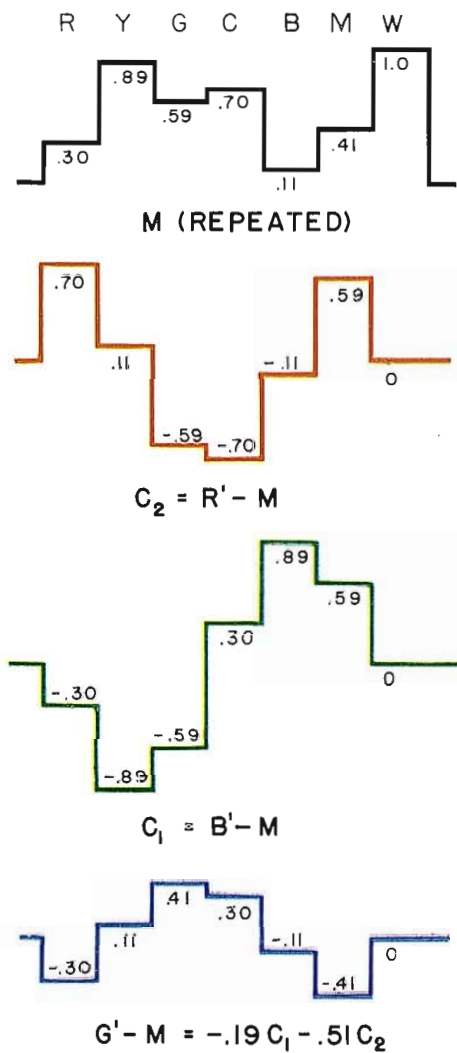
FIG. 21. Bar-pattern waveforms showing the derivation of the composite signal for a compatible system in which the (R-M) and (B-M) signal levels are reduced to 88% and 49%, respectively, to limit overshoots to 33%.
