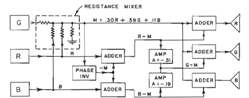
FIG. 9. Block diagram showing complete matrix operations for compatible color television system.
