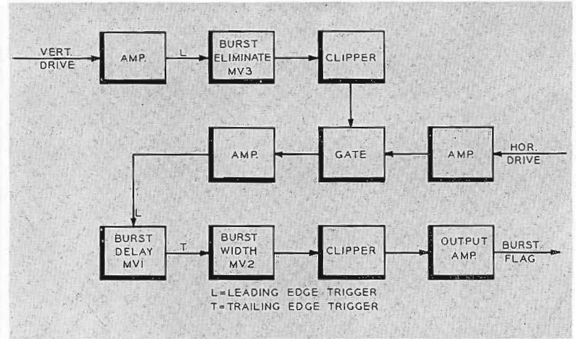
FIG. 4. Block diagram showing the functions of the Burst Flag Generator.
