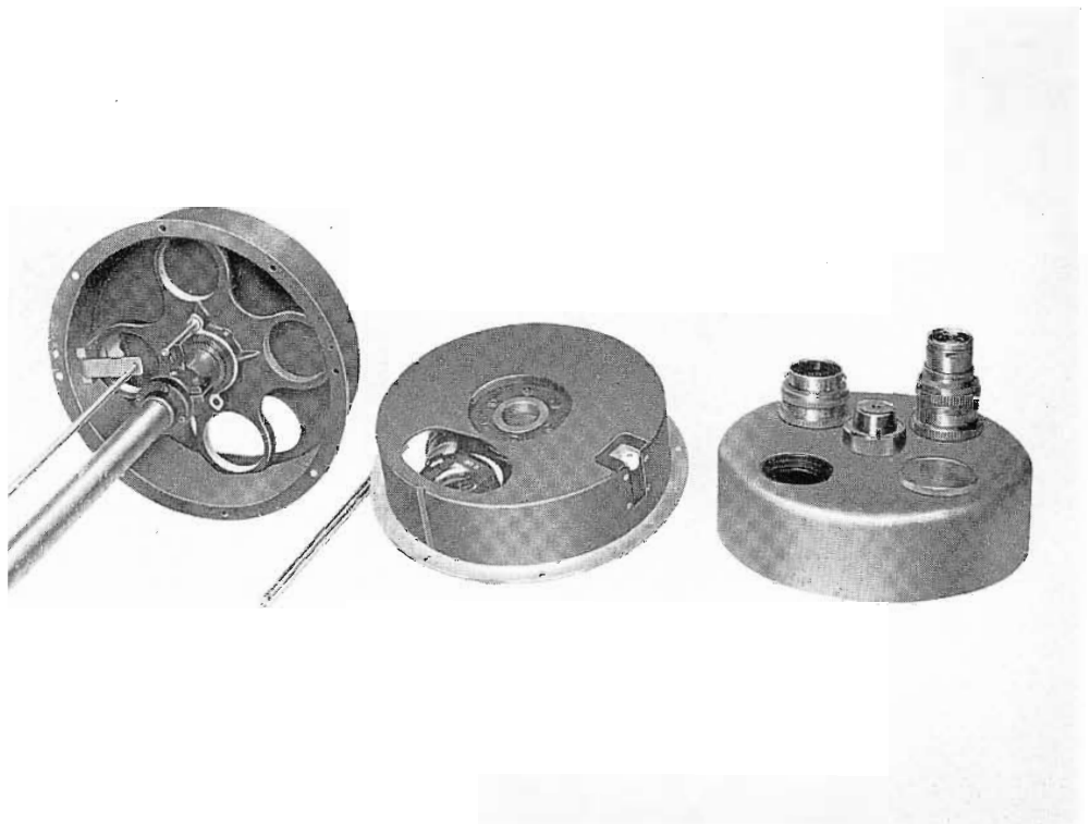
FIG. 9. Details of the lens turret assembly showing the rotating turret drum, the stationary turret drum and the lens turret assemblies.
