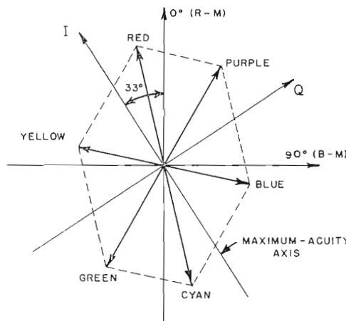
FIG. 24. Vector diagram showing location of maximum acuity axis.
