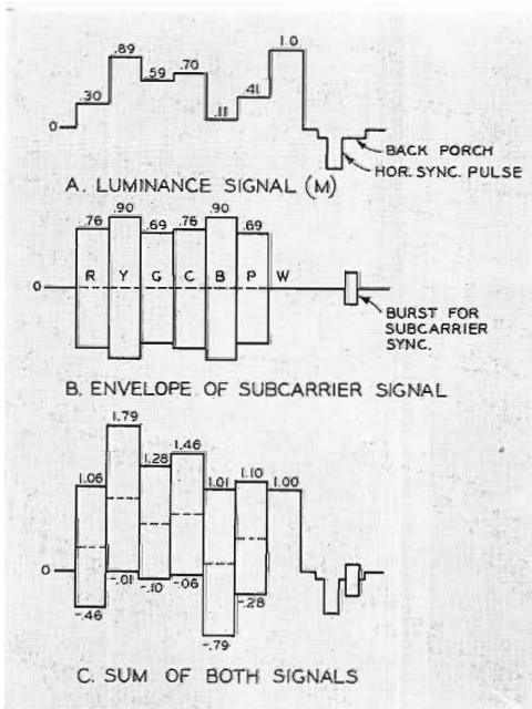
FIG. 20. Bar-pattern waveforms showing the derivation of the composite signal for a system in which all components are transmitted at unity level relative to each other.
