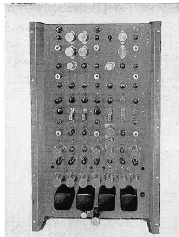
FIG. 13. Channel amplifier chassis.
