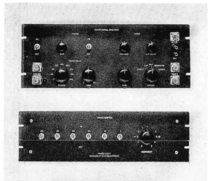
FIG. 4. The Color Signal Analyzer is used for measuring phase of subcarrier frequency. Along with Linearity Checker it is used for phase intermodulation checks.
