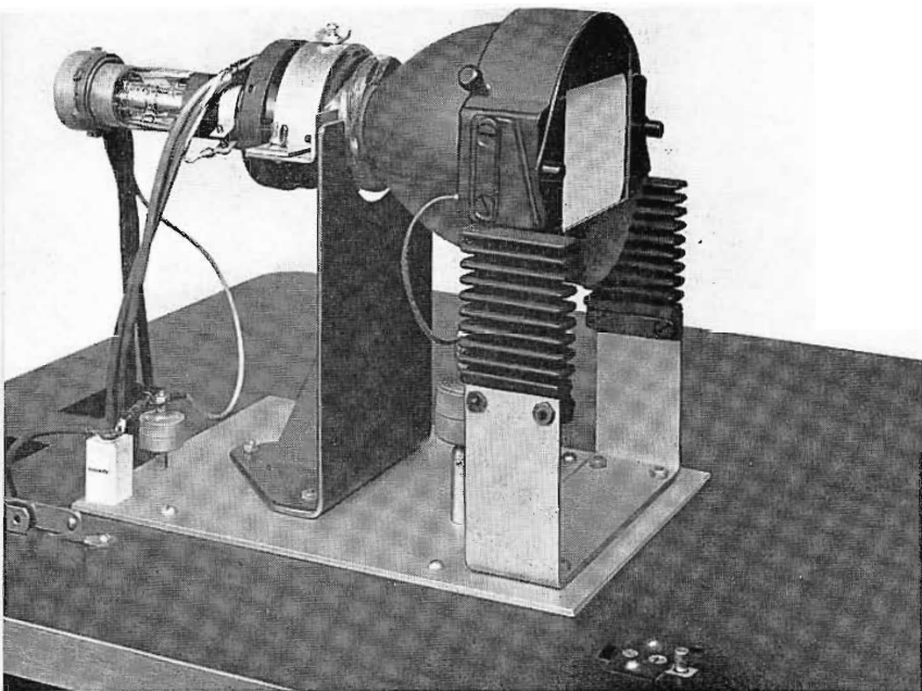
FIG. 4. Kinescope and mounting. Kinescope is used as light source for scanning slide transparency. See Fig. 7 for Kinescope position in relation to overall system.
