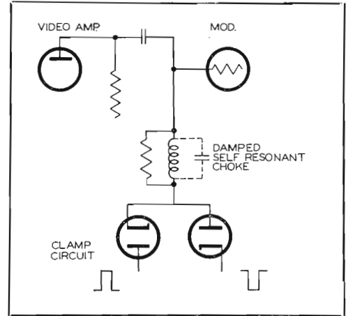
FIG. 9. Modification to "soften" clamp circuit. Damped self-resonant choke is inserted between clamp diodes and modulator grid.
