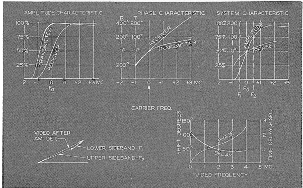
FIG. 11. Relation between transmitter and receiver amplitude and phase characteristics and the required phase characteristic of the low frequency delay equalizer.
