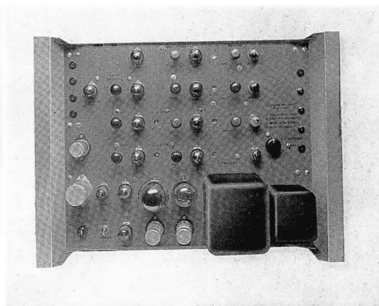
FIG. 3. The Color Bar Generator provides a standard signal, relatively free of residual imperfections. Its signal is analogous to the monoscope signal in monochrome television.
