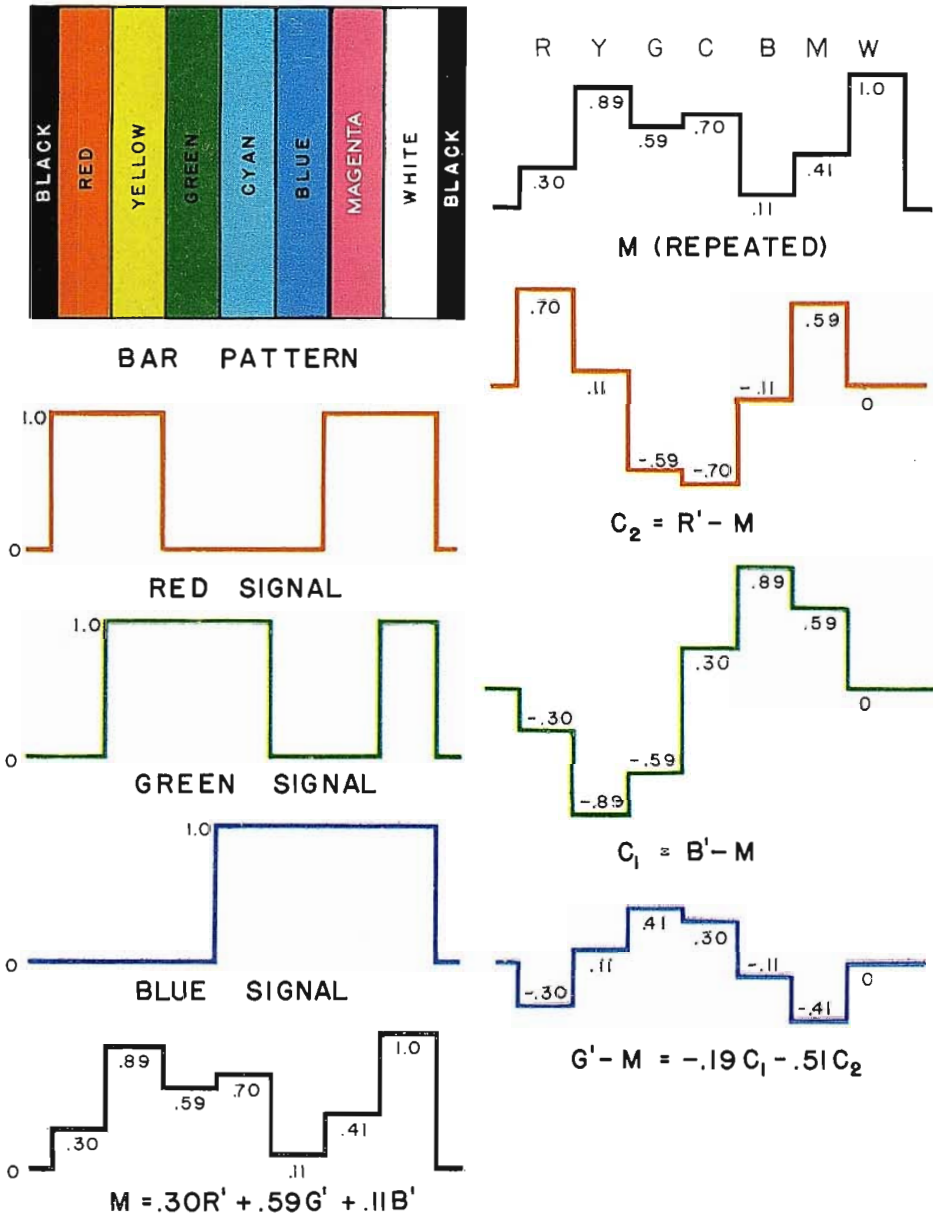
FIG. 19 (above). A typical bar pattern and horizontal-frequency waveforms illustrating the operation of a compatible color television system.
