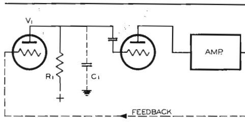
FIG. 8. Simplified schematic of feedback video amplifier.
