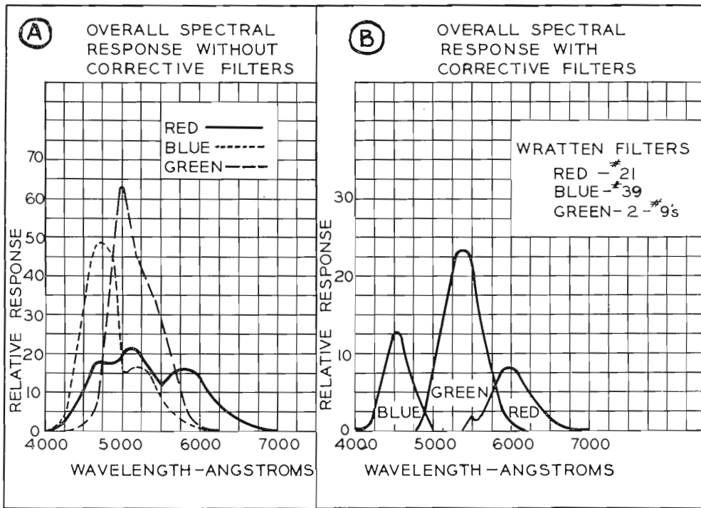
FIGS. 10A and B. Overall spectral response curves.
