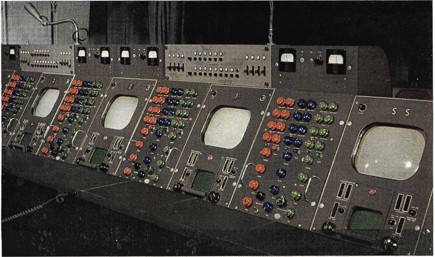
FIG. 1. Camera Control Console in the control room of NBC's Colonial Theatre Color Studio. Four RCA Color Cameras are controlled from this position. Each camera "chain" includes a camera control unit (the panels with a large number of knobs) and a modified Type TM-5B master monitor (used for monochrome monitoring).
