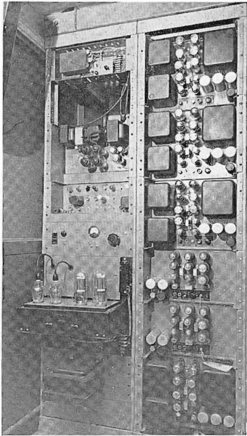
FIG. 3. View of the power supplies used for the fast pull-down projector equipment. Rack at left supplies power to the projector motor.
