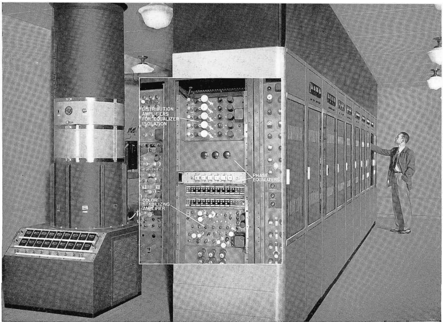
FIG. 1. Conversion to color mainly consists of adding some rack mounted input equipment as shown in the inset of the above photo. This equipment is installed external to the transmitter.
