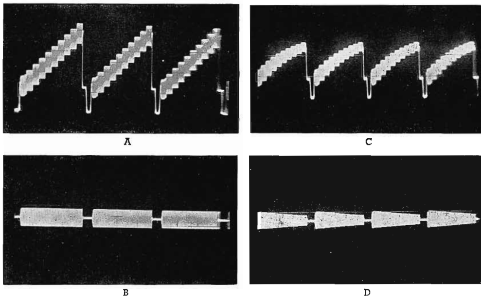
FIGS. 19A, B, C, D. Waveforms produced by linearity checker and transmitter. A. Waveform produced by linearity checker. B. High frequency component of linearity checker waveform. C. Waveform out of demodulator. D. High frequency component of demodulator output.
