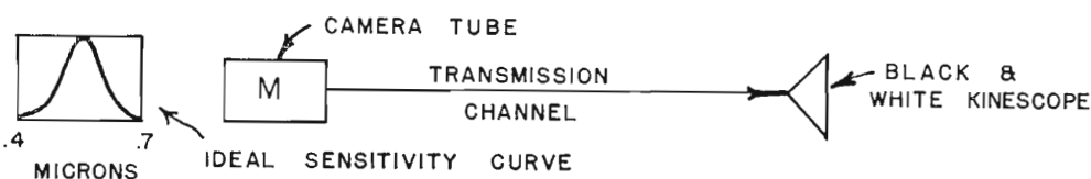
FIG. 4. Simplified block diagram for a monochrome television system.
