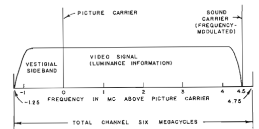
FIG. 10. Sketch of a standard television broadcast channel.
