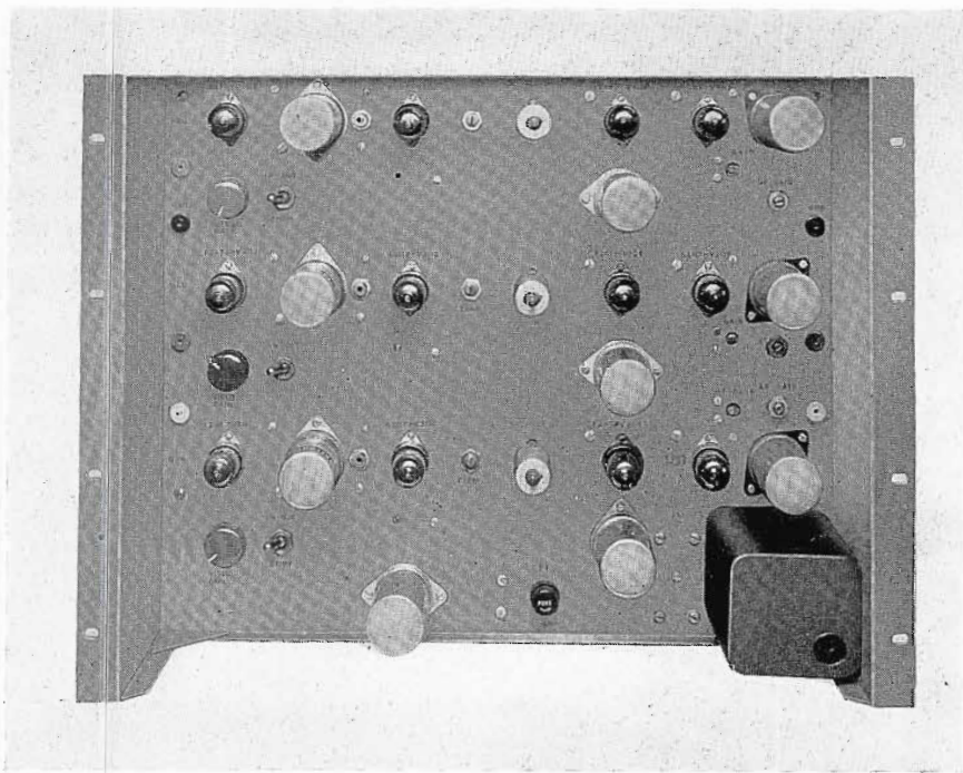
FIG. 13 (below). Aperture Compensator. Serves to restore high-frequency video information—providing greater picture detail.
