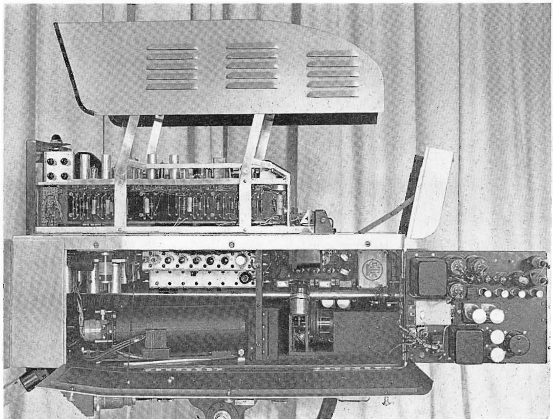
FIG. 6. Rear view of RCA Color Camera with viewing hood in place.
