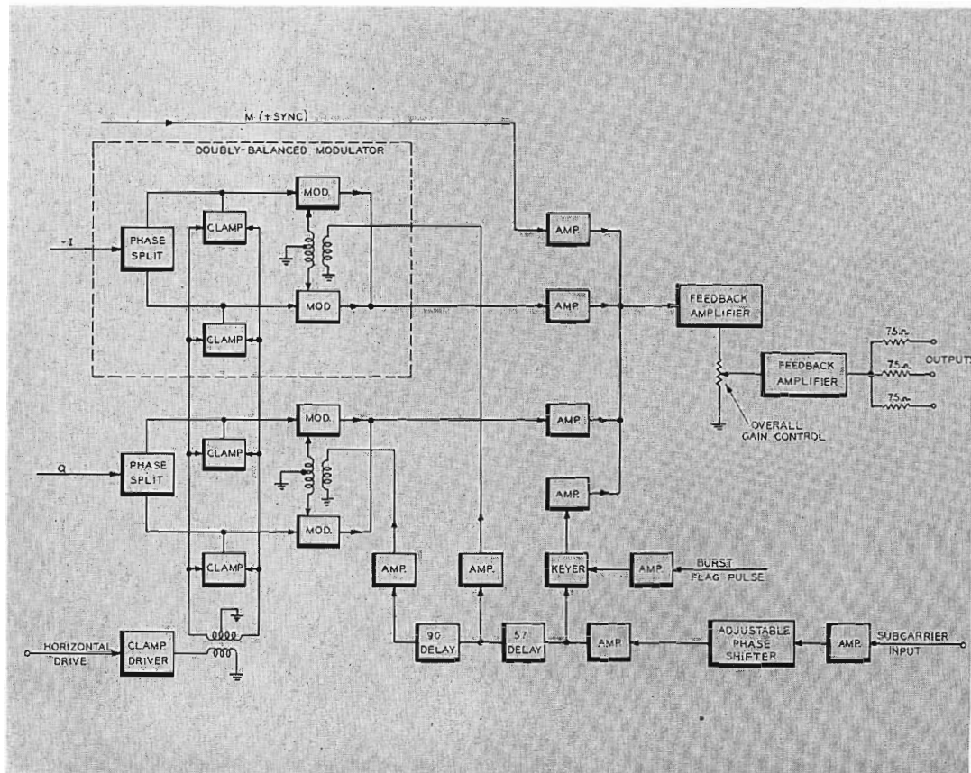
FIG. 3. Block diagram for the multiplexer section of a Colorplexer.
