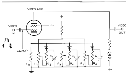
FIG. 17. Schematic diagram of non-linear amplifier, employed in the color stabilizing amplifier.
