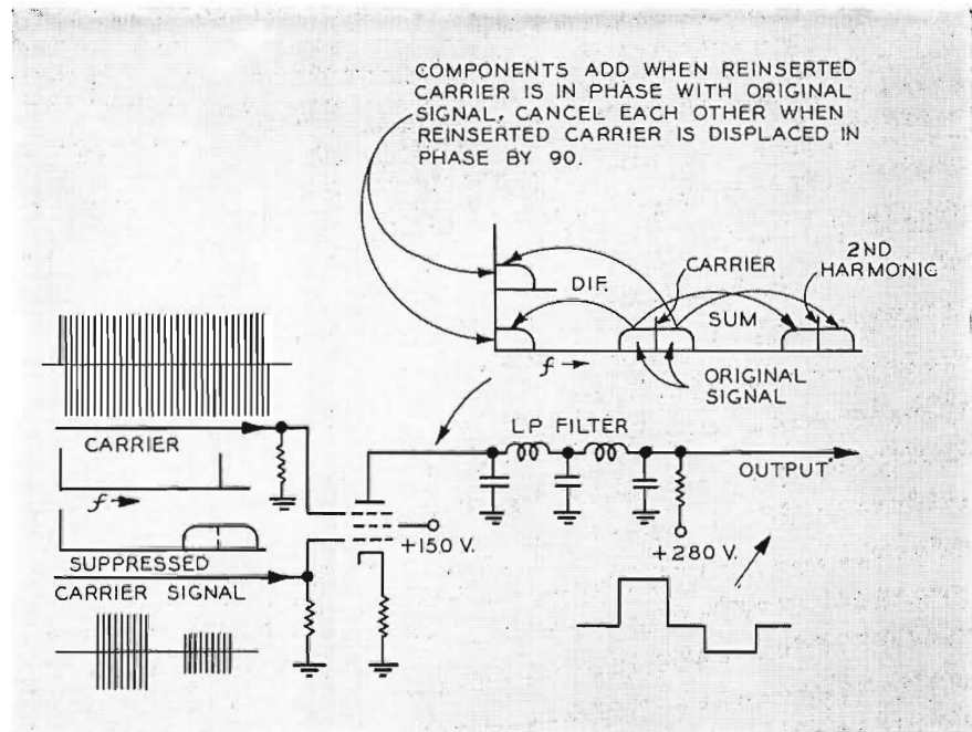
FIG. 16. Simplified schematic for a suppressor-grid modulator used as a synchronous detector.
